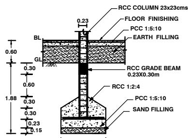
FOUNDATION DETAILS
