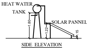
SIDE ELEVATION
