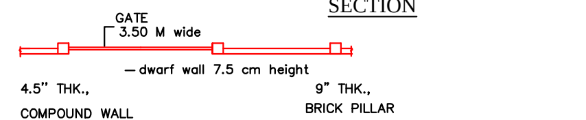
COMPOUND WALL PLAN
