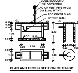
PLAN AND CROSS SECTION OF ST&SP
