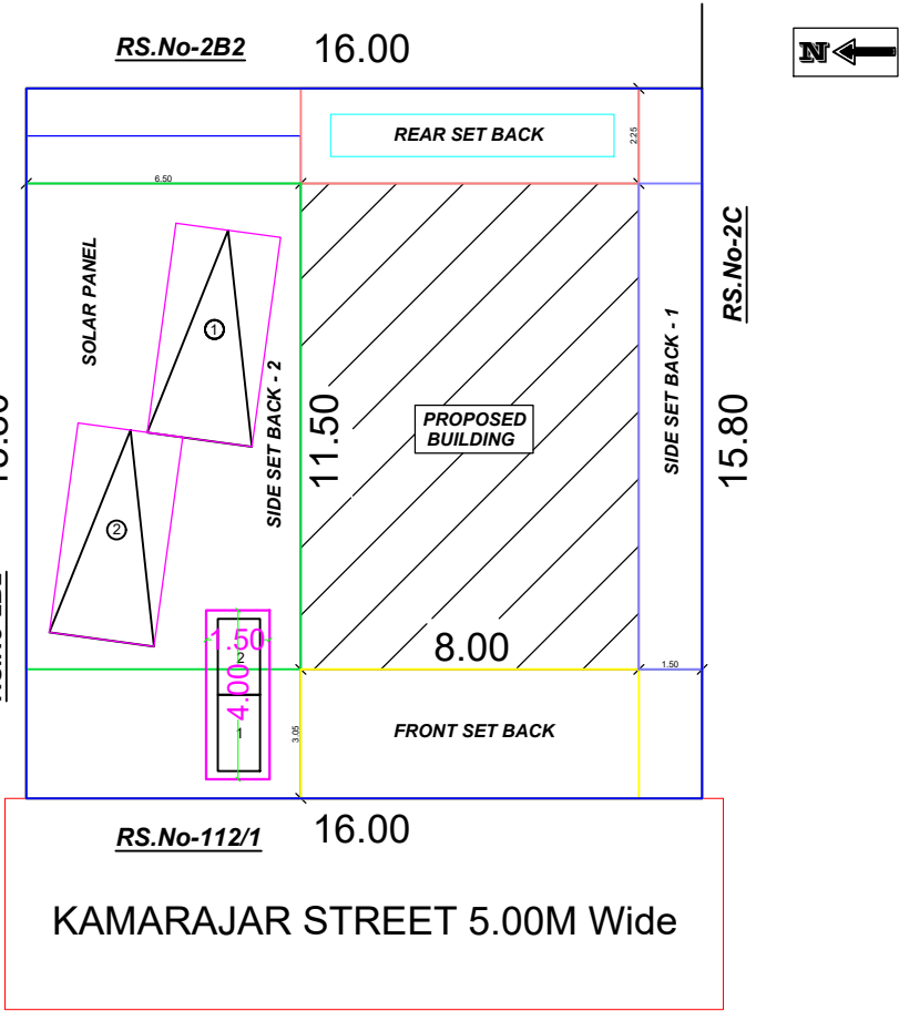
SITE PLAN
