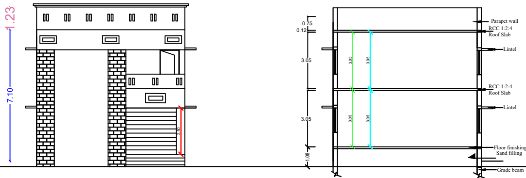
FRONT ELEVATION
