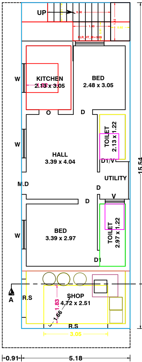
EXI. & PRO.GROUND FLOOR PLAN
