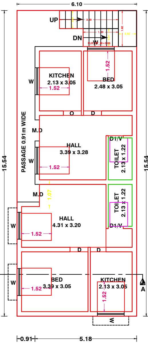
PRO.FIRST FLOOR PLAN
