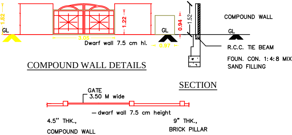
COMPOUND WALL PLAN
