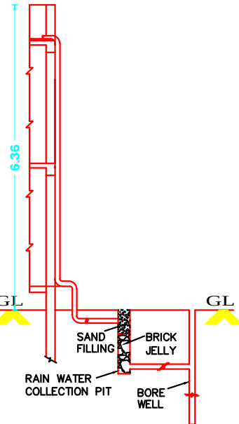
RAIN WATER HARVESTING SYSTEM RWH_CAPACITY_L=1000LTRS
