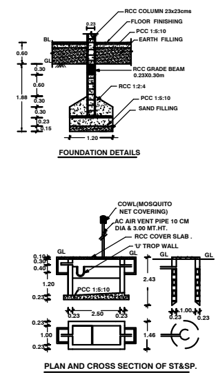
FOUNDATION DETAILS
