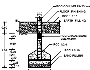
FOUNDATION DETAILS
