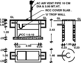
PLAN AND CROSS SECTION OF ST&P.
