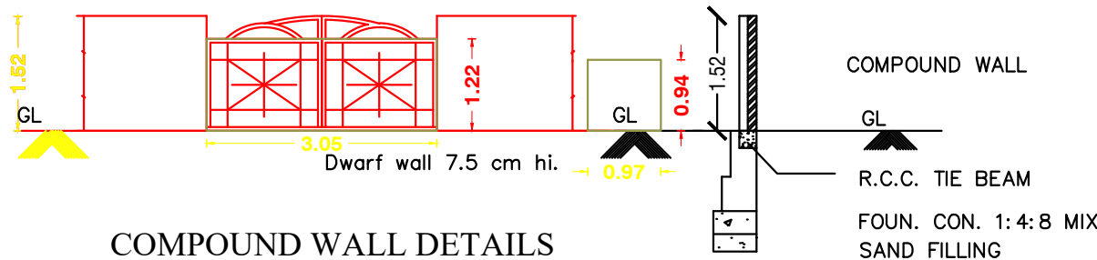
SECTION
