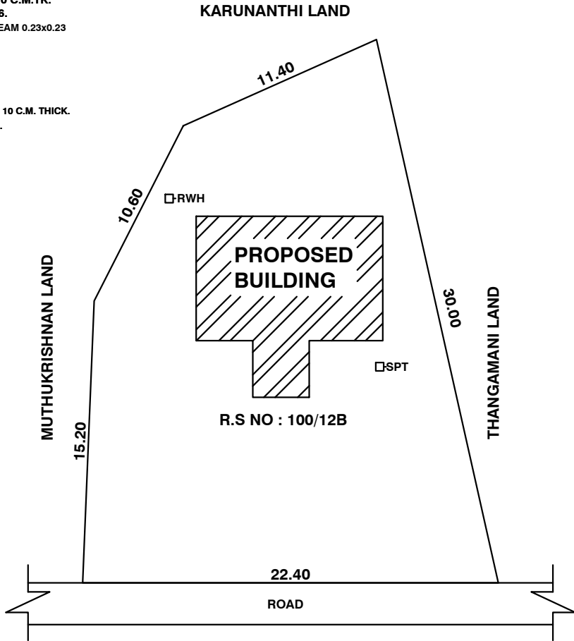
SITE PLAN
