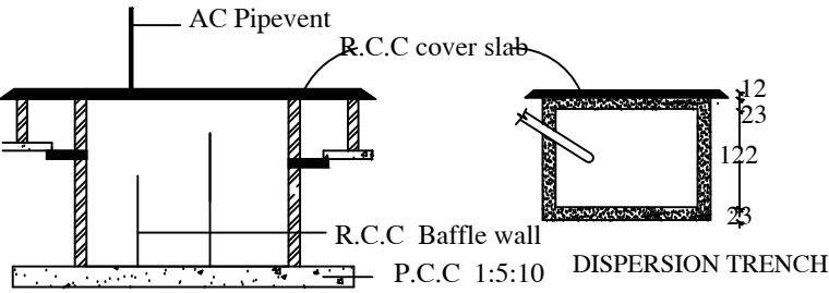
SEPTIC TANK
