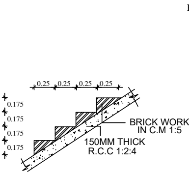
STAIRCASE DETAILS NOT TO SCALE
