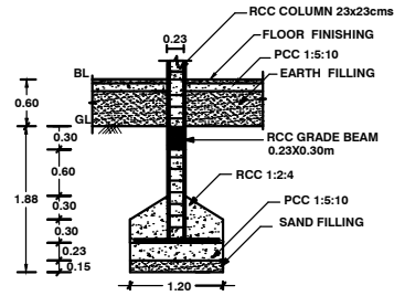
FOUNDATION DETAILS
