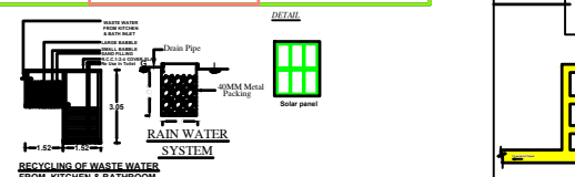
RECYCLING OF WASTE WATER FROM KITCHEN & BATHROOM
