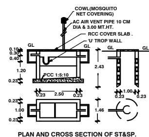
PLAN AND CROSS SECTION OF STAIR.
