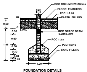
FOUNDATION DETAILS
