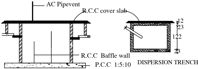
SEPTIC TANK
