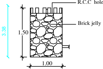
COLLECTING RAIN WATER PIT Not to Scale
