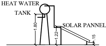
SIDE ELEVATION
