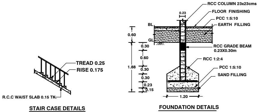
STAIR CASE DETAILS
