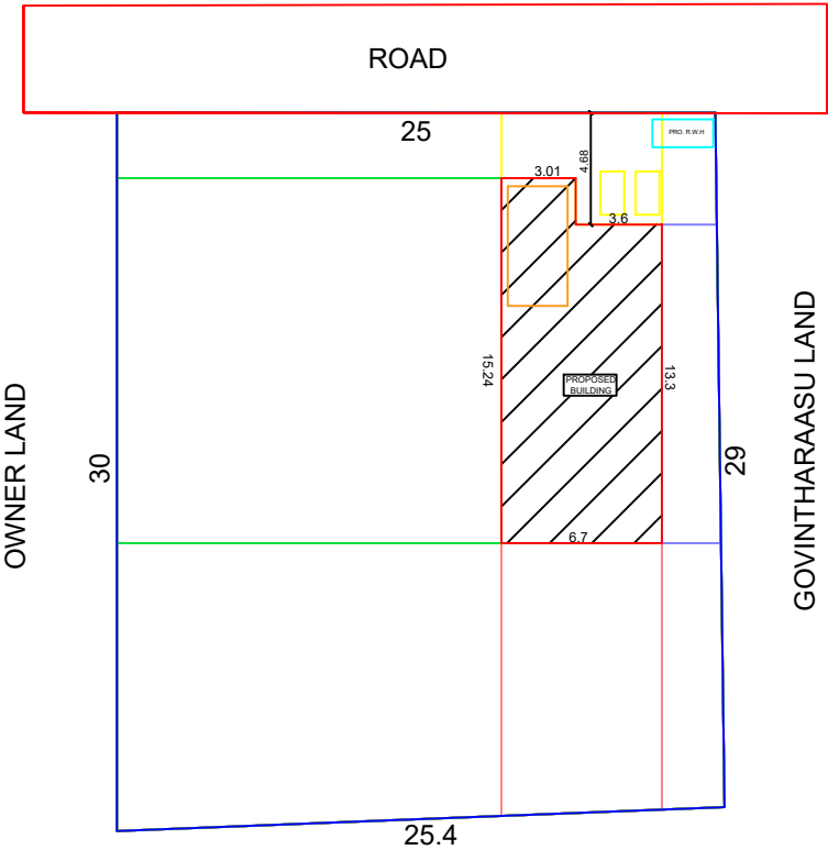
SITE PLAN
