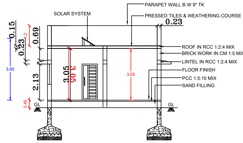
CROSS SECTION AB
