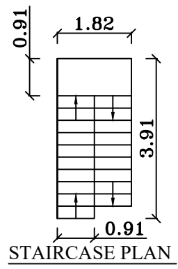
STAIRCASE PLAN
