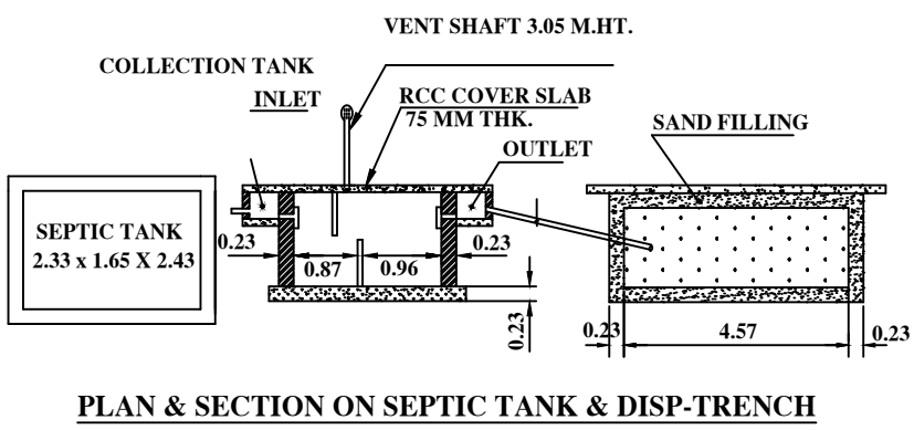
PLAN & SECTION ON SEPTIC TANK & DISP.TRENCH
