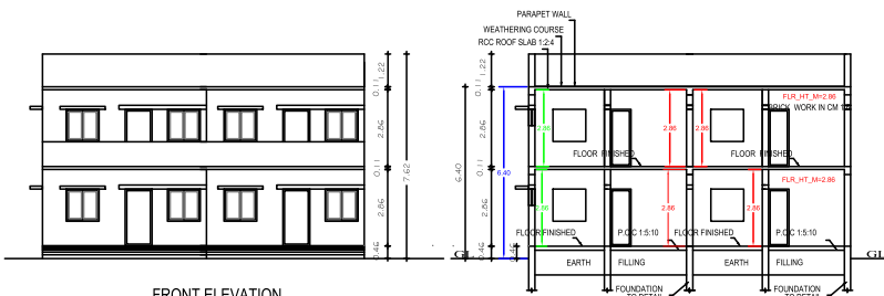
SECTION "A-B"
