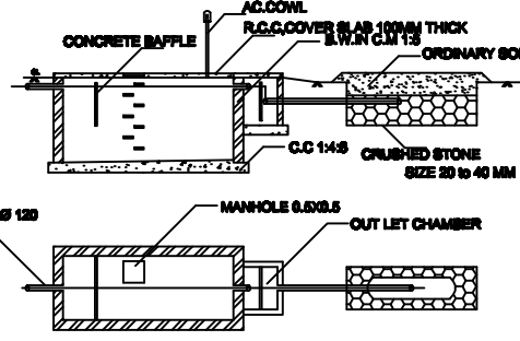
SEPTIC TANK WITH DISPERSION TRENCH
