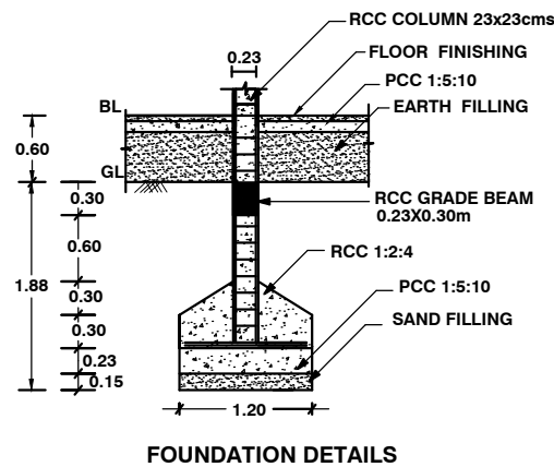
FOUNDATION DETAILS
