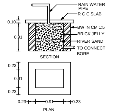
RAIN WATER COLLECTION TANK (SCALE 1:50)
