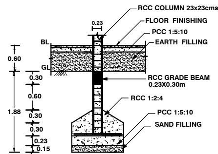
FOUNDATION DETAILS
