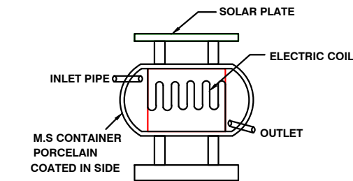
SOLAR SYSTEM
