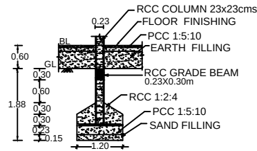
FOUNDATION DETAILS
