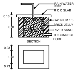
RAIN WATER COLLECTION TANK
