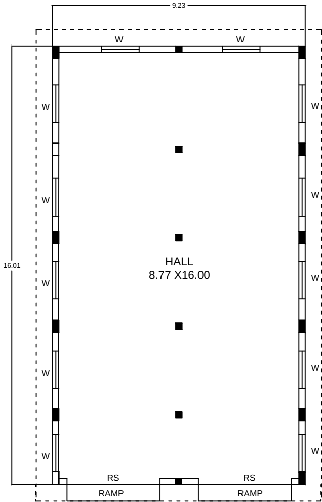
EXI.GROUND FLOOR PLAN
