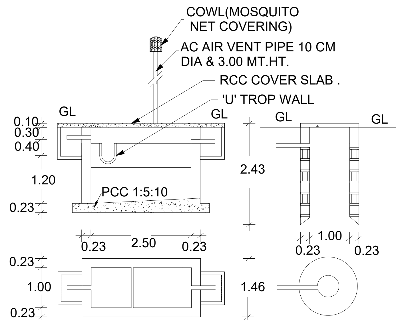
PLAN AND CROSS SECTION OF ST&SP.
