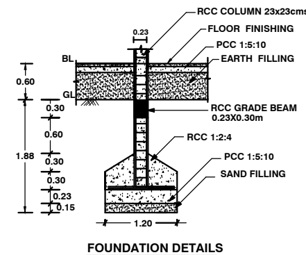
FOUNDATION DETAILS
