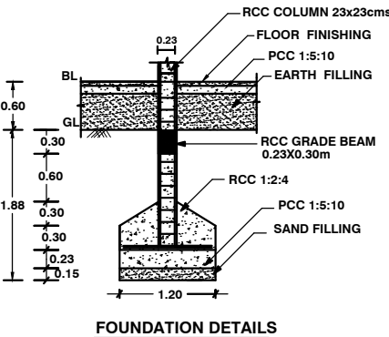
FOUNDATION DETAILS
