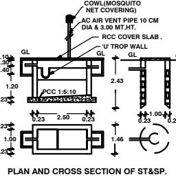
PLAN AND CROSS SECTION OF ST&SP
