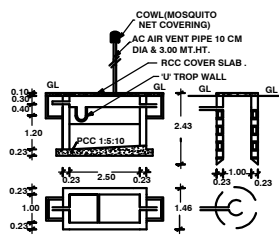
PLAN AND CROSS SECTION OF ST&SP.
