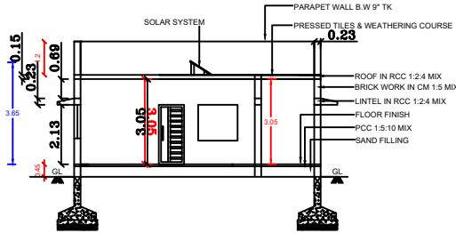
CROSS SECTION AB
