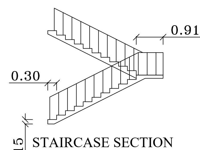
5 | STAIRCASE SECTION
