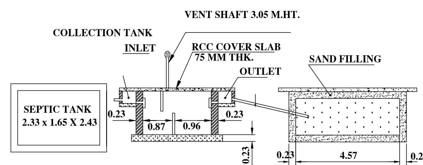
PLAN & SECTION ON SEPTIC TANK & DISP-TRENCH
