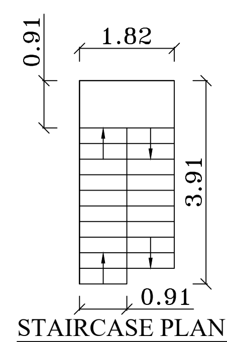
STAIRCASE PLAN
