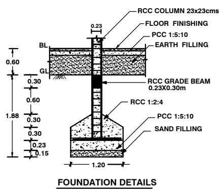
FOUNDATION DETAILS
