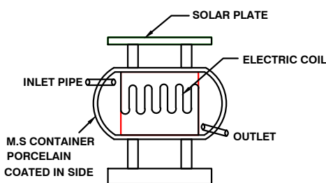
SOLAR SYSTEM
