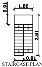
STAIRCASE PLAN
