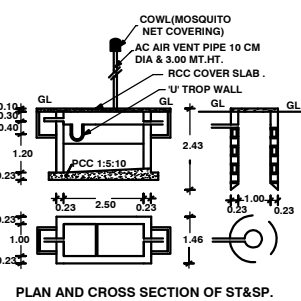
PLAN AND CROSS SECTION OF ST&SP.
