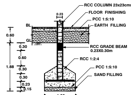
FOUNDATION DETAILS
