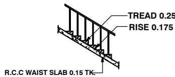
STAIR CASE DETAILS
