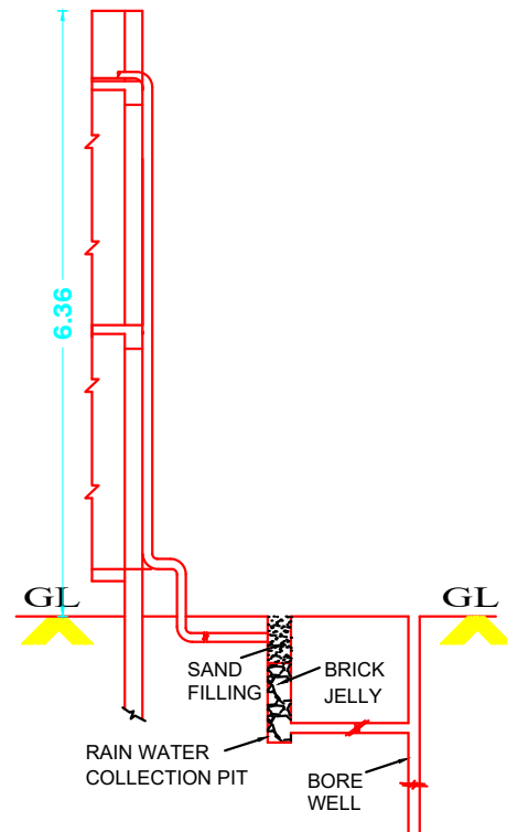
RAIN WATER HARVESTING SYSTEM RWH_CAPACITY_L=1000LTRS
