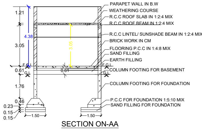
SECTION ON-AA
