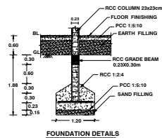
FOUNDATION DETAILS
