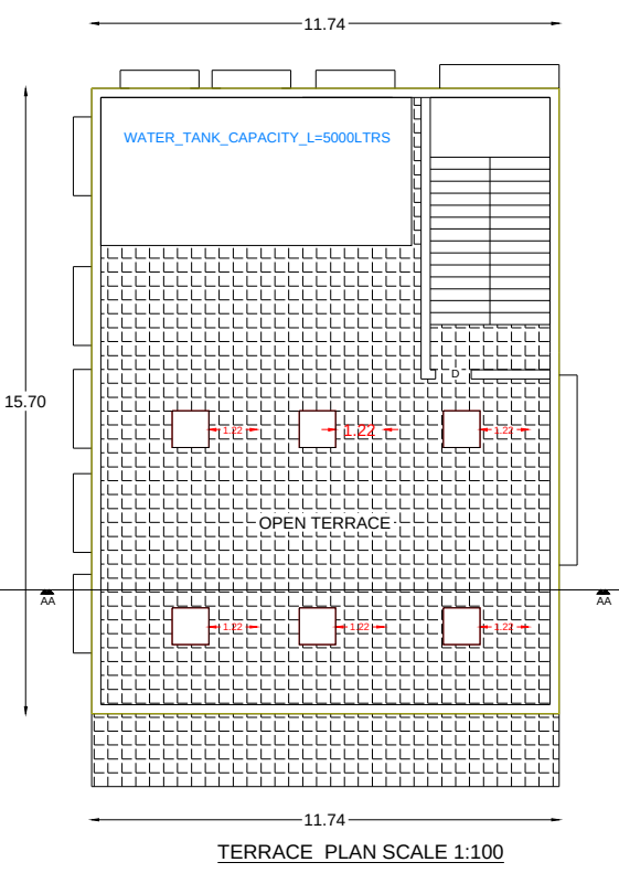
TERRACE PLAN SCALE 1:100
