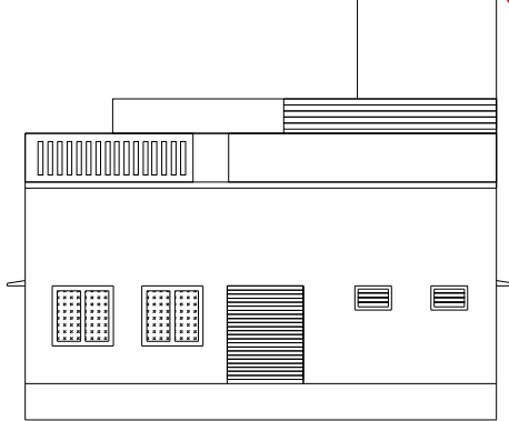
ELEVATION SCALE 1:100
