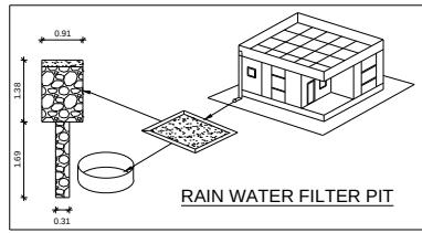
RAIN WATER FILTER PIT
