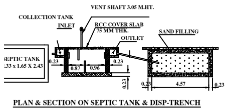
PLAN & SECTION ON SEPTIC TANK & DISP-TRENCH
