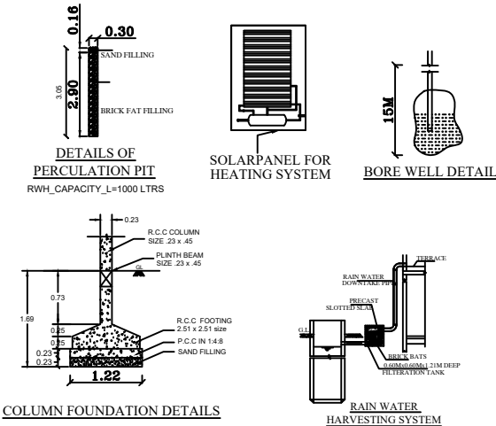
COLUMN FOUNDATION DETAILS
