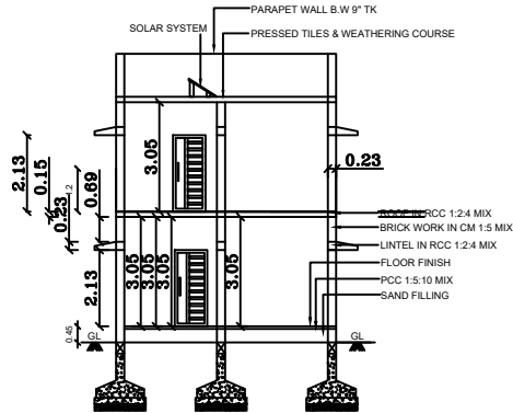
CROSS SECTION AB
