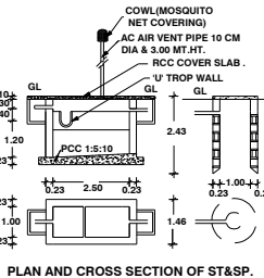
PLAN AND CROSS SECTION OF ST&SP.
