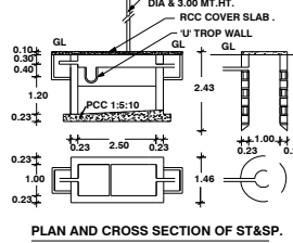
PLAN AND CROSS SECTION OF STAIR.
