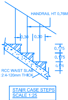
STAIR CASE STEPS SCALE 1:25
