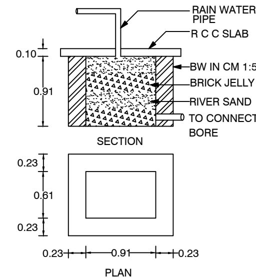
RAIN WATER COLLECTION TANK (SCALE 1:50)
