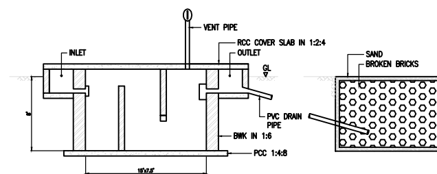
SECTIONAL DETAILS OF SEPTIC TANK & DISPERSION TRENCH
