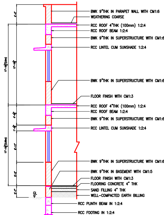
TYPICAL BUILDING SECTION
