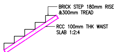
TYPICAL STAIR SECTION
