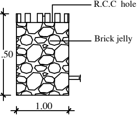
COLLECTING RAIN WATER PIT Not to Scale
