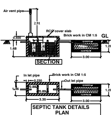
SEPTIC TANK DETAILS PLAN
