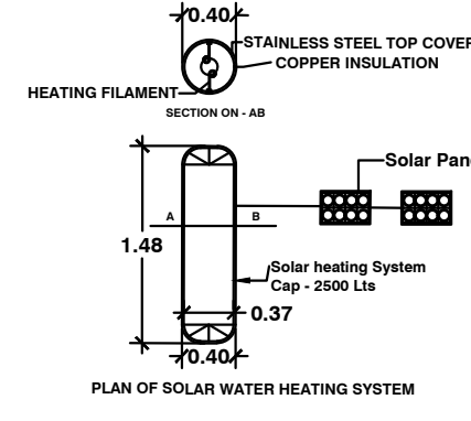
PLAN OF SOLAR WATER HEATING SYSTEM SCALE 1:50
