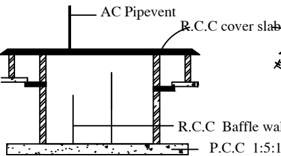
SEPTIC TANK
