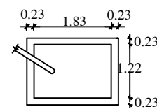
DISPERSION TRENCH
