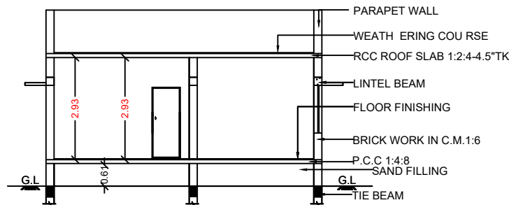
SECTION AT AB
