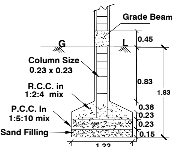
COLUMN DETAILS
