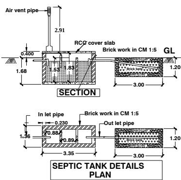
SEPTIC TANK DETAILS PLAN
