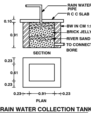
RAIN WATER COLLECTION TANK
