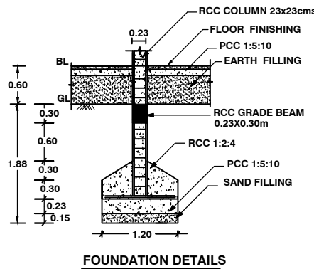
FOUNDATION DETAILS
