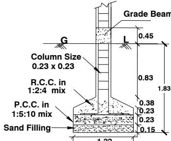
COLUMN DETAILS
