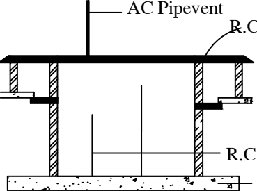
SEPTIC TANK
