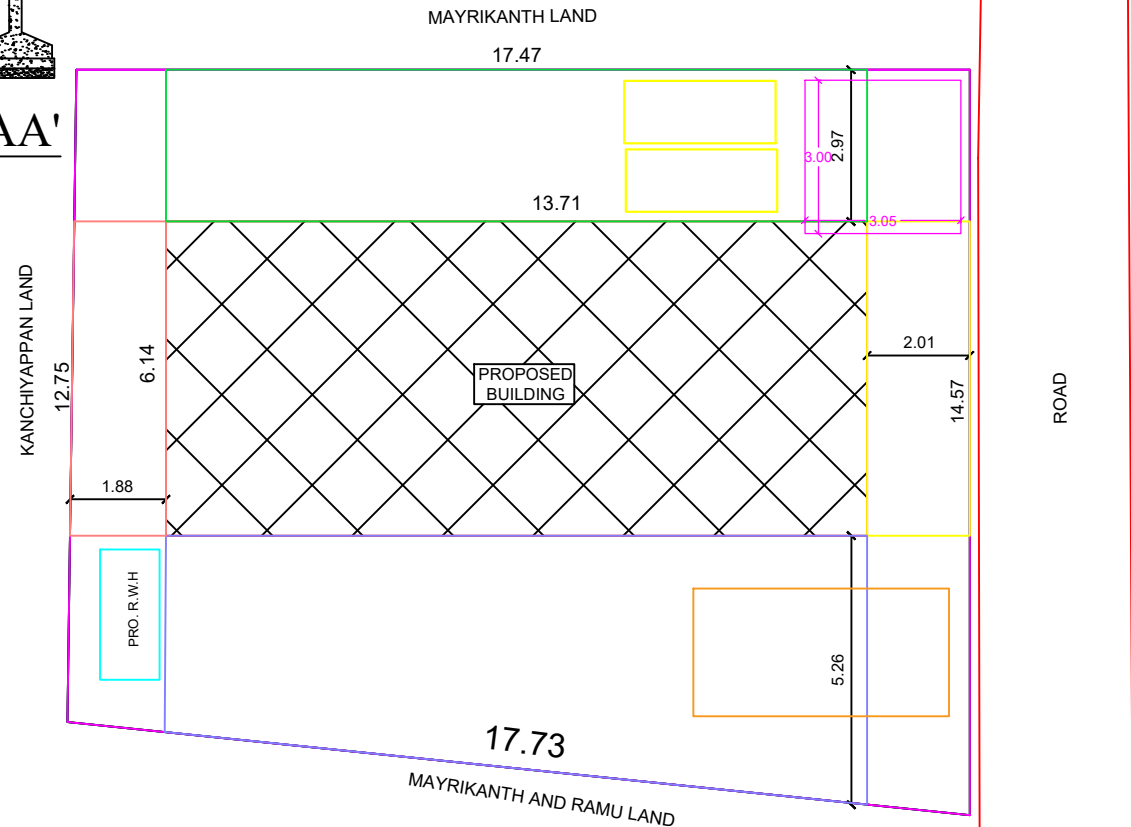
SITE PLAN
